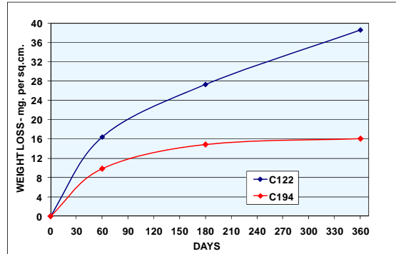
Figure 2 – Corrosion of Alloys C194 and C122 in a 3.4% NaCl solution at 5 fps.
