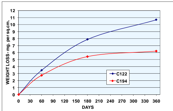
Figure 1 – Corrosion of Alloys C194 and C122 in New Haven Potable Water at 7fps.
